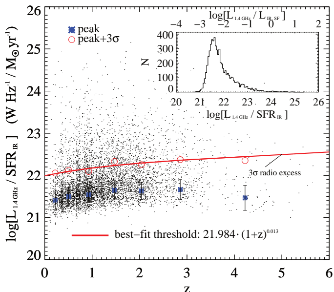
Fig. 4: Distribution of the ratio between L_{1.4\text{ GHz}} and \text{SFR}_{\text{IR}} as a function of redshift (black points) for sources not classified as HLAGN (79% of our sample). The blue filled circles (and errors) indicate the peak (and dispersion) of the Gaussian distribution identified in a given redshift bin, while the corresponding 3\sigma deviation is set by the red open circles. The red solid line indicates the redshift-dependent threshold derived by fitting the open circles at each redshift bin. Sources above the red line are identified as “low to moderate radiative luminosity AGN” (hereafter MLAGN) via radio excess. The full histogram of L_{1.4\text{ GHz}}/\text{SFR}_{\text{IR}} is shown in the top right corner.
