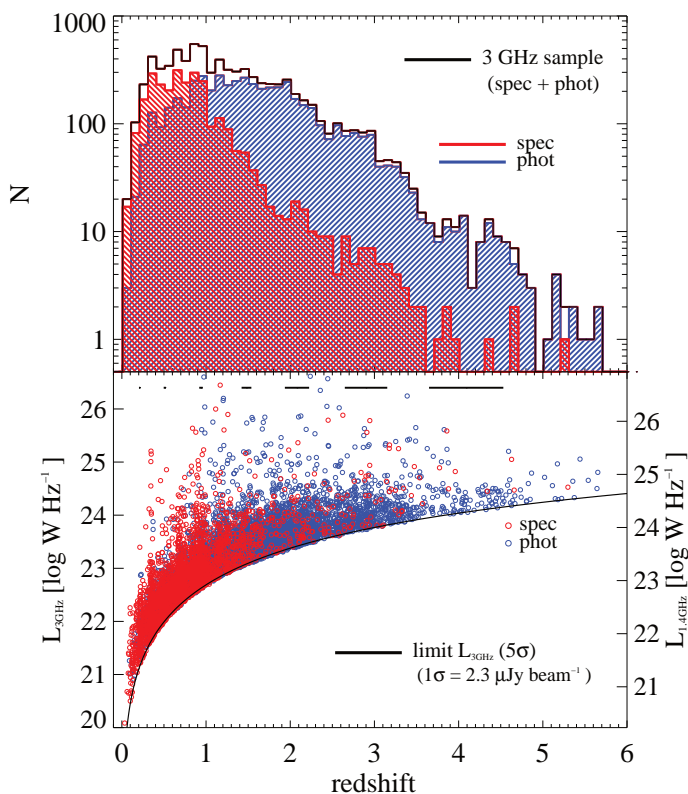
Fig. 1: Top panel: redshift distribution of our 7 729 radio sources. Spectroscopic and photometric redshifts are shown in red and blue, respectively, while the black line is the sum of the two. The scale of the y axis is logarithmic. Bottom panel: circles show the rest-frame 3 GHz luminosity as a function of redshift, both spectroscopic (red) and photometric (blue). The horizontal bars indicate the average \pm 1\sigma uncertainty range of the photometric redshifts in the various redshift bins. The corresponding 1.4 GHz luminosity (scaled by using \alpha = -0.7 ) is shown for comparison on the right y axis. The black solid line indicates the 5\sigma luminosity limit at 3 GHz.
