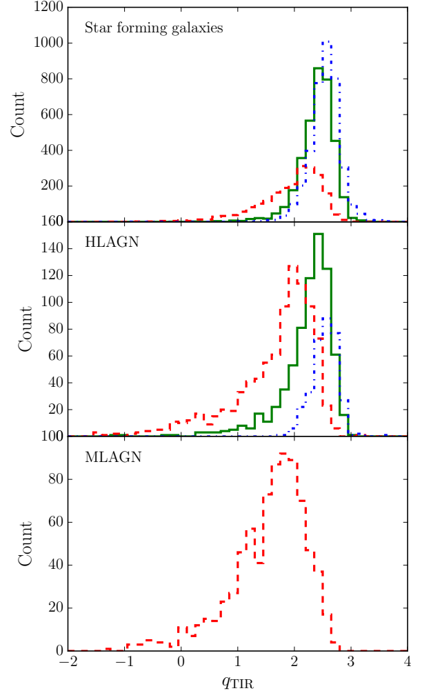
Fig. 17. Distribution of direct q_{TIR} measurements (solid green line), lower limits (blue dot-dashed line) upper limits (red dashed line) shown separately for the populations of star-forming galaxies, HLAGN and MLAGN, as indicated.
