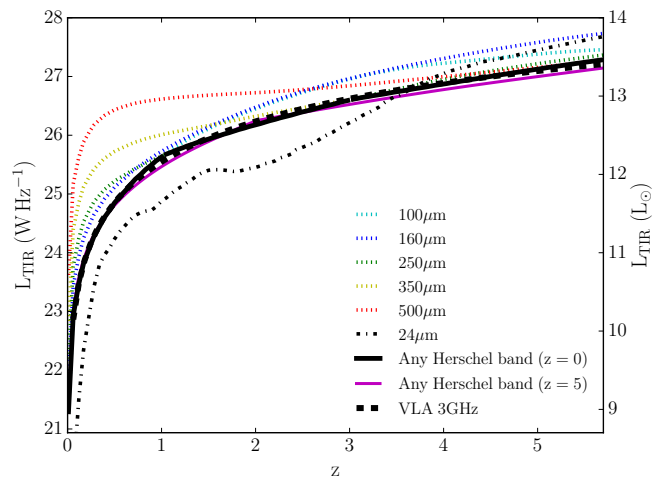
Fig. 8. Total infrared luminosity limit of various data sets. Dashed, coloured lines show the limit in various Herschel bands assuming a z = 0 galaxy template (see text, Section 2.3.4, for details). The black line traces the lowest coloured line at each redshift and represents the sensitivity limit of the infrared-selected sample. The magenta line is the equivalent using z = 5 templates. The 5\sigma sensitivity limit of the Spitzer 24\,\mu\text{m} data is shown as the black dot-dashed line. The sensitivity limit of the VLA 3 GHz Large Project (dashed black line) is also shown, assuming q_{\text{TIR}} = 2.64 (Bell 2003) and a radio spectral index of \alpha = -0.7 .
