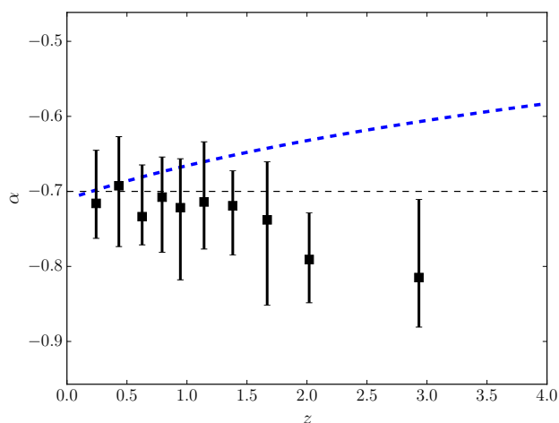
Fig. 21. Radio spectral index of sources detected at both 3 GHz and 1.4 GHz as a function of redshift. As in Figure 3, the median values within each redshift bin, derived from a single-censored survival analysis, are shown by the black squares. The predicted evolution in the spectral index due to the contamination of free-free emission based on the M82 model of Condon (1992) is shown by the thick, dashed blue line. Our assumed value of \alpha = -0.7 for non-detections at 1.4 GHz is shown by the black dashed line.
