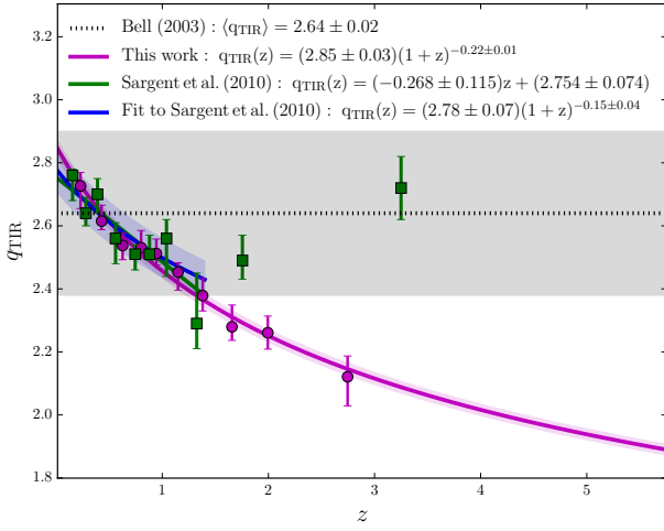
Fig. 12. Evolution of q_{\text{TIR}} in comparison with the results of Sargent et al. (2010). The magenta points and fit show the results from this work using a full survival analysis, as in Figure 9, however a spectral index of \alpha = -0.8 has now been assumed for objects not detected at 1.4 GHz. The measurements of Sargent et al. (2010) and their linear fit are shown by the green points and line. A power-law evolution to the individual measurements of Sargent et al. (2010) is shown by the blue line, for ease of comparison. The shaded magenta and blue regions show the 1\sigma uncertainty regions calculated by propagating the errors on the corresponding fitting parameters. The local measurement and spread (grey shading) of Bell (2003) are also shown.
