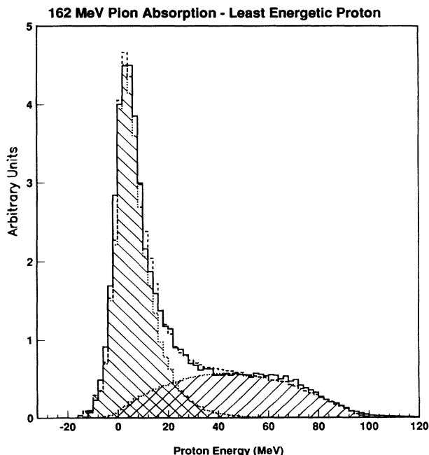
FIG. 2. The energy of the least energetic outgoing proton from the absorption of 162 MeV \pi^+ on ^3\text{He} . The solid line is the data, the dotted lines are the results of the 2NA (the low energy peak) and the 3NA (the broad spectrum) simulations, and the dashed line is the sum of the two. The simulations include the effect of the detector's acceptance.
