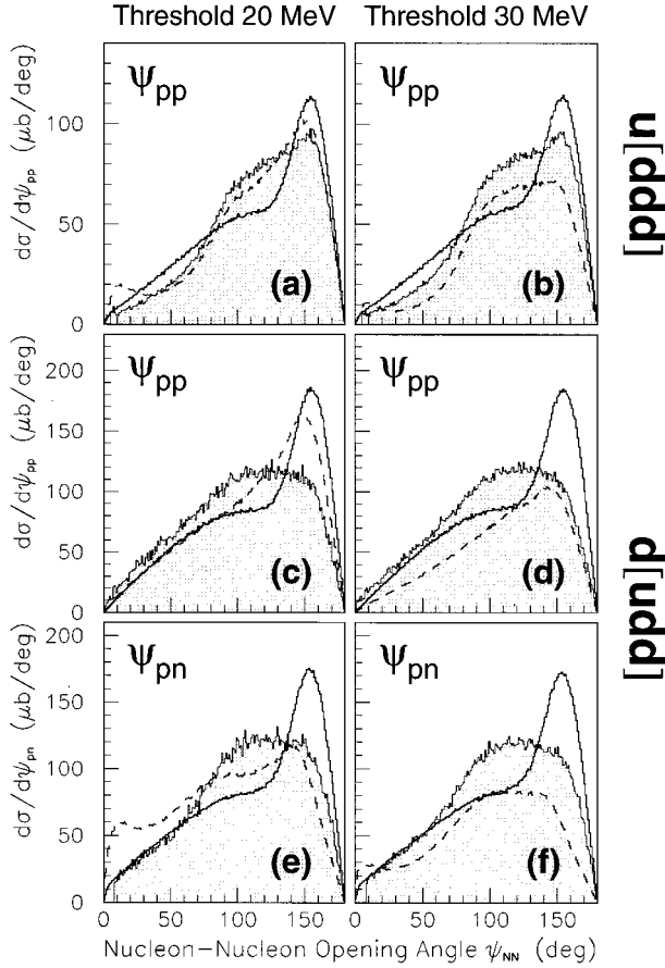
FIG. 4. Nucleon-nucleon laboratory opening angles \psi_{NN} of the reaction \pi^+{}^4\text{He} \rightarrow pppn at 239 MeV. Left column [(a),(c),(e)]: T_{N1-N3} > 20 MeV; T_{N4} \leq 20 MeV. Right column [(b),(d),(f)]: T_{N1-N3} > 30 MeV; T_{N4} \leq 30 MeV. The shaded areas are the acceptance corrected data, and the dashed and solid lines the results of HFSI and ISI simulations, respectively, normalized to the yield with the 20 MeV threshold; the results of the simulations for the 30 MeV data retain this normalization but with the higher threshold applied. (a)+(b): \psi_{pp} of the [ppp]n channel (all three combinations added) compared to the \text{ISI}_{(ppp)n} and the \text{HFSI}_{(ppp)n} models. (c)+(d): \psi_{pp} of the [ppn]p channel (all three combinations added) compared to the \text{ISI}_{(ppn)p} and the \text{HFSI}_{(ppn)p} models. (e)+(f): \psi_{pn} of the [ppn]p channel (all three combinations added) compared to the \text{ISI}_{(ppn)p}^{\text{SCX}} and the \text{HFSI}_{(ppn)p} models.
