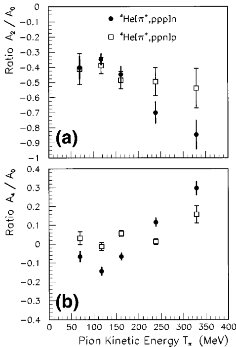
FIG. 7. Coefficient ratios A_2/A_0 (a) and A_4/A_0 (b) of the fits of Legendre polynomials [Eq. (5.1)] to the plane angle \xi for the [ppp]n (solid dots) and the [ppn]p (open squares) channels with a 20 MeV threshold.
