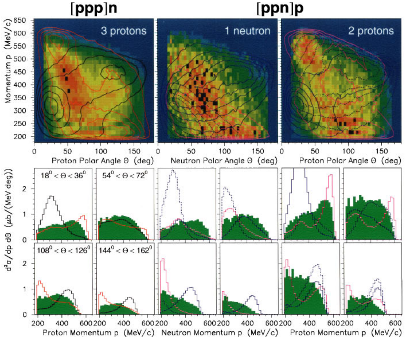
FIG. 3. (Color). \theta_N vs p_N correlations (upper row) of the reaction \pi^+{}^4\text{He} \rightarrow pppn at 118 MeV and sliced projections (lower rows) of the momentum p_N within selected angular regions. The labels and color codes are the same as those of Fig. 2.
