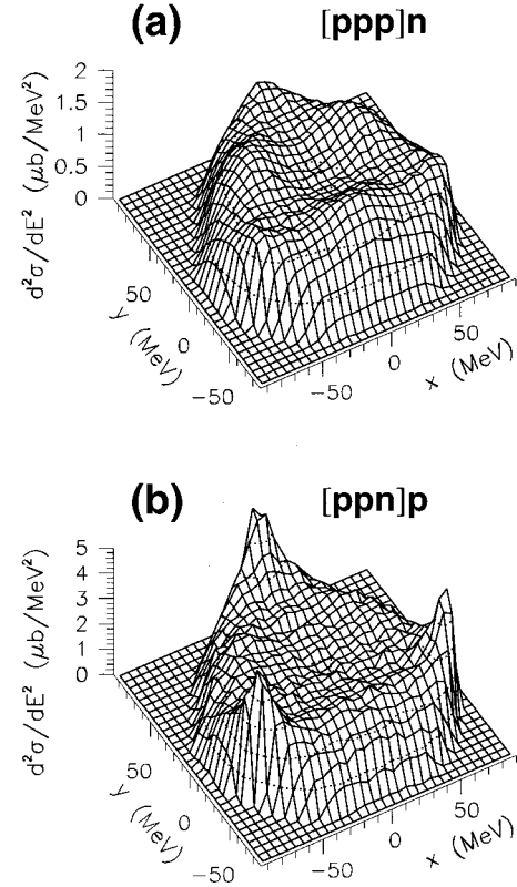
FIG. 5. Triangular Dalitz plots of 3NA on {}^4\text{He} for the channels [ppp]n (a) and [ppn]p (b). The incident pion energy was 162 MeV. The sharp peaks in the [ppn]p channel are due to pn SFSI. The variables are defined as x = (T_1 - T_2)/\sqrt{3} and y = T_3 - Q/3 , with Q = T_1 + T_2 + T_3 and T_i the kinetic energy of the nucleon i in the 3N c.m. system.
