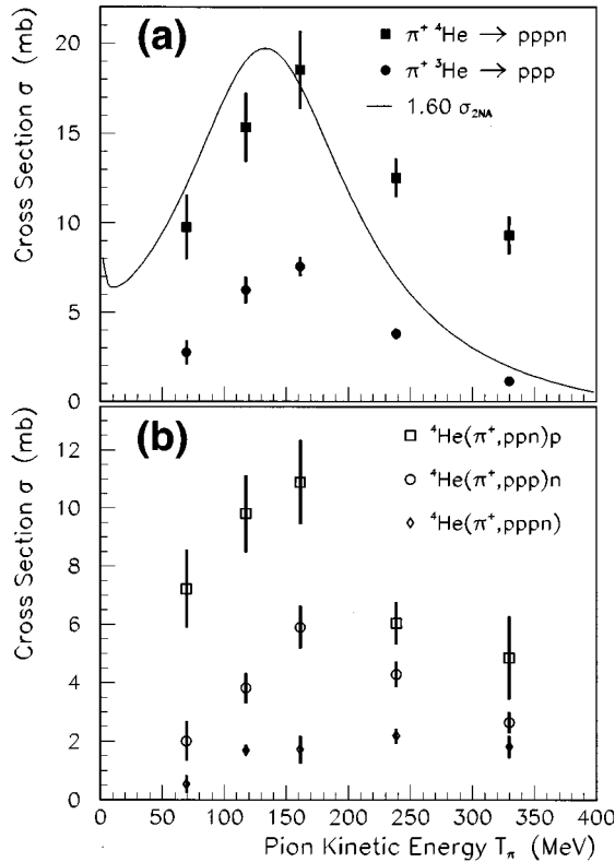
FIG. 15. (a) Multinucleon cross sections \sigma_{ppp} and \sigma_{pppn} for the reactions \pi^+{}^3\text{He} \rightarrow ppp and \pi^+{}^4\text{He} \rightarrow pppn , respectively. The curve represents the 2NA cross section (arbitrarily normalized) as parametrized in Ref. [37]. (b) Decomposition of the {}^4\text{He} pppn absorption yield into the 3NA absorption channels 3NA( ppp ) and 3NA( ppn ), and the 4NA absorption channel 4NA( pppn ).
