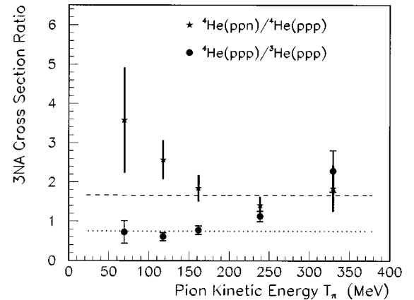
FIG. 16. Ratios between the 3NA cross sections \sigma_{ppp}^{4\text{He}} and \sigma_{ppp}^{3\text{He}} and between the two isospin different 3NA channels 3NA( ppn ) and 3NA( ppp ) of {}^4\text{He} . The experimental data are compared to the isospin ratios deduced in Ref. [19]: \sigma_{ppp}^{4\text{He}}/\sigma_{ppp}^{3\text{He}} (dotted line) and \sigma_{ppn}/\sigma_{ppp} of {}^4\text{He} (dashed line).
