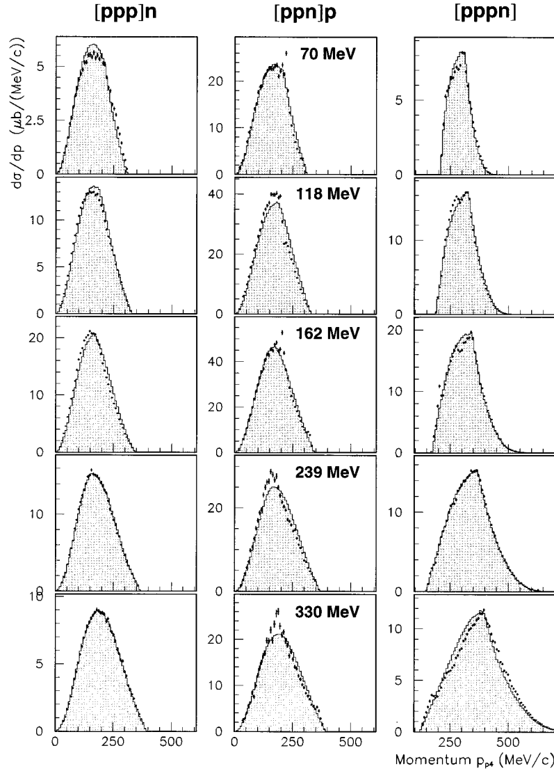
FIG. 12. Distributions over the momentum p_{p4} of the fourth particle in the c.m. system of the other three nucleons for the reaction \pi^+{}^4\text{He} \rightarrow pppn for incident pion energies of 70, 118, 162, 239, and 330 MeV (from the top) with a threshold of 20 MeV. For further information see Fig. 8.
