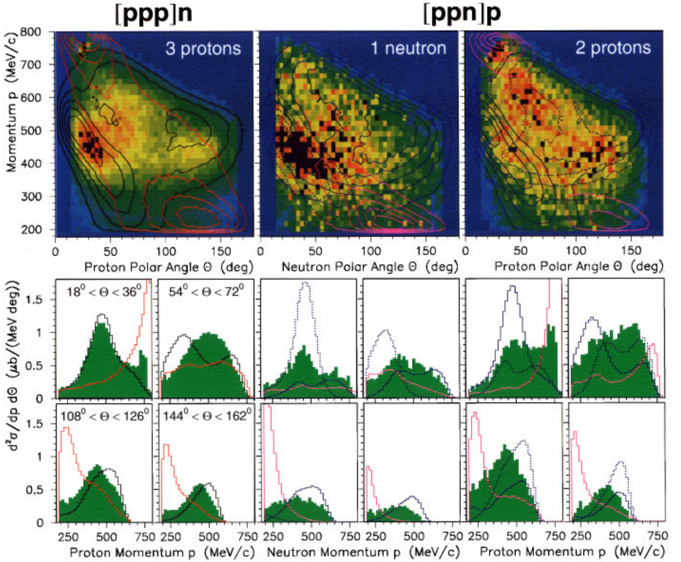
FIG. 2. (Color). \theta_N vs p_N correlations (upper row) of the reaction \pi^+{}^4\text{He} \rightarrow pppn at 239 MeV and sliced projections (lower rows) of the momentum p_N within selected angular regions. All histograms are corrected for acceptance. Each of the simulations is individually normalized to the full content of the two-dimensional histograms of the experimental data. The z axis of the two-dimensional plots is arbitrarily scaled; the color sequence is linearly increasing from blue, green, yellow, brown, to black. The four one-dimensional histograms below each correlation are momentum projections for the angular intervals 18^\circ < \theta_N < 36^\circ , 54^\circ < \theta_N < 72^\circ , 108^\circ < \theta_N < 126^\circ , and 144^\circ < \theta_N < 162^\circ . The green areas of the one-dimensional plots are the data corrected for acceptance. Left column: the three protons of the [ppp]n channel compared to the \text{ISI}_{(ppp)n} (black line) and the \text{HFSI}_{(ppp)n} (red line) models. Middle column: the neutron of the [ppn]p channel compared to the \text{ISI}_{(ppn)p} (dotted blue line), the \text{ISI}_{(ppn)p}^{\text{SCX}} (solid blue line), and the \text{HFSI}_{(ppn)p} (pink line) models. Right column: the two fast protons of the [ppn]p channel compared to the \text{ISI}_{(ppn)p}^{\text{SCX}} (solid blue line), the \text{ISI}_{(ppn)p} (dotted blue line), and the \text{HFSI}_{(ppn)p} (pink line) models.
