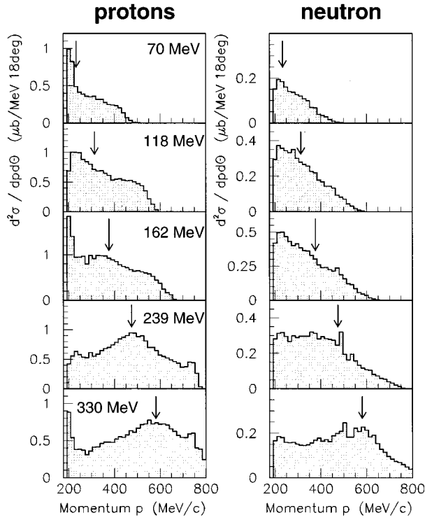
FIG. 6. Proton (left) and neutron (right) momentum yields of the pion absorption channel [pppn] (for definition see Sec. IV D) on {}^4\text{He} within an angular region of 18^\circ – 36^\circ for the five incident pion energies 70, 118, 162, 239, and 330 MeV. Always all three protons in the given range are plotted in the left histograms. The arrows indicate the positions of a nucleon in quasifree \pi N kinematics.
