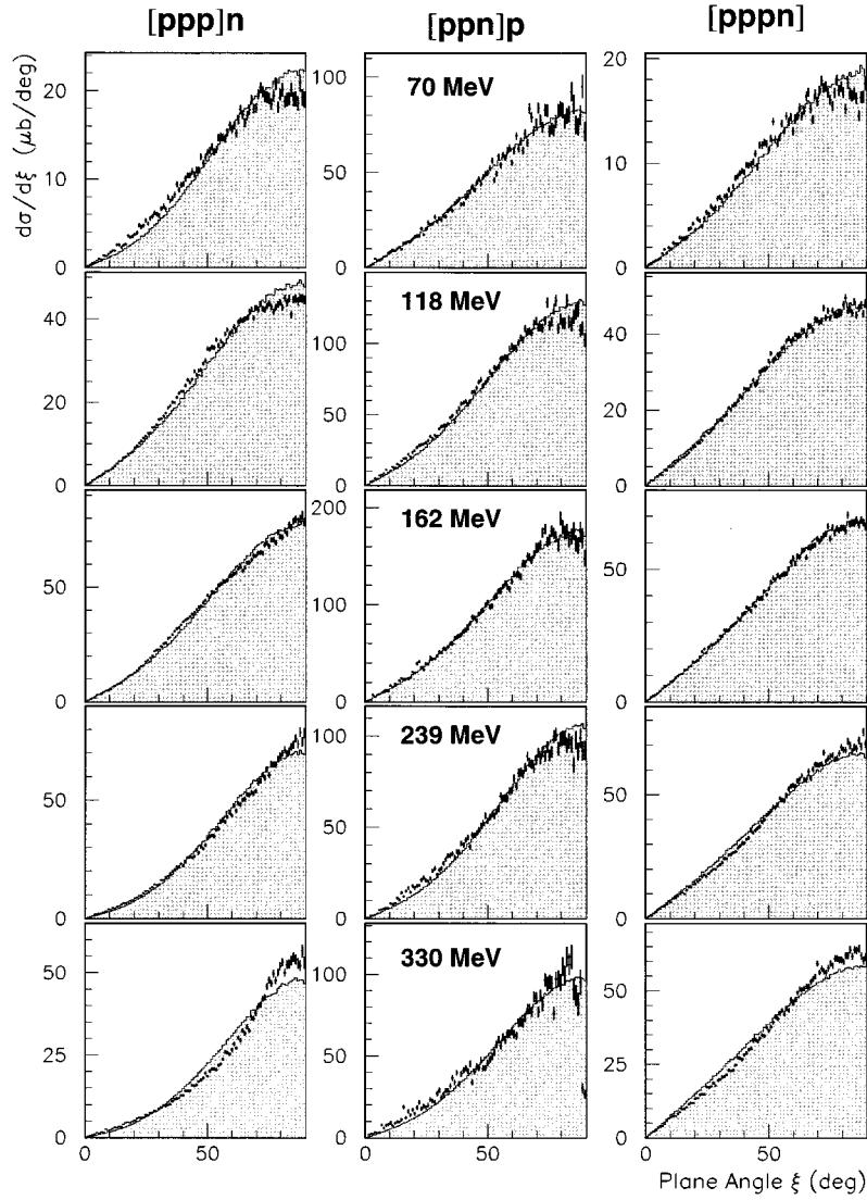
FIG. 8. Distributions over the plane angle \xi for the reaction \pi^+{}^4\text{He} \rightarrow pppn for incident pion energies of 70, 118, 162, 239, and 330 MeV (from the top) with a threshold of 20 MeV. The data are the dots with error bars, the fitted sums of the simulations are the shaded areas. The columns show the channels [ppp]n (left), [ppn]p (middle), and [pppn] (right). Normalization uncertainties are not included in the error bars.
