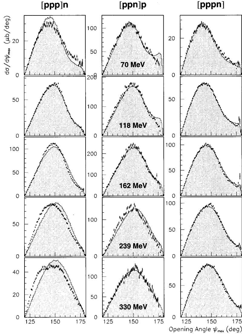
FIG. 11. Distributions over the maximum opening angle \psi_{\max} for the reaction \pi^+{}^4\text{He} \rightarrow pppn for incident pion energies of 70, 118, 162, 239, and 330 MeV (from the top) with a threshold of 20 MeV. For further information see Fig. 8.
