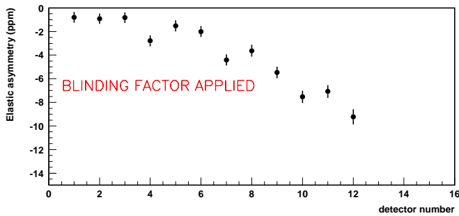
Figure 1. G^0 forward angle preliminary result. Elastic asymmetry as a function of detector number is displayed. Lower detectors indicate lower Q^2 and higher detectors indicate higher Q^2 .
