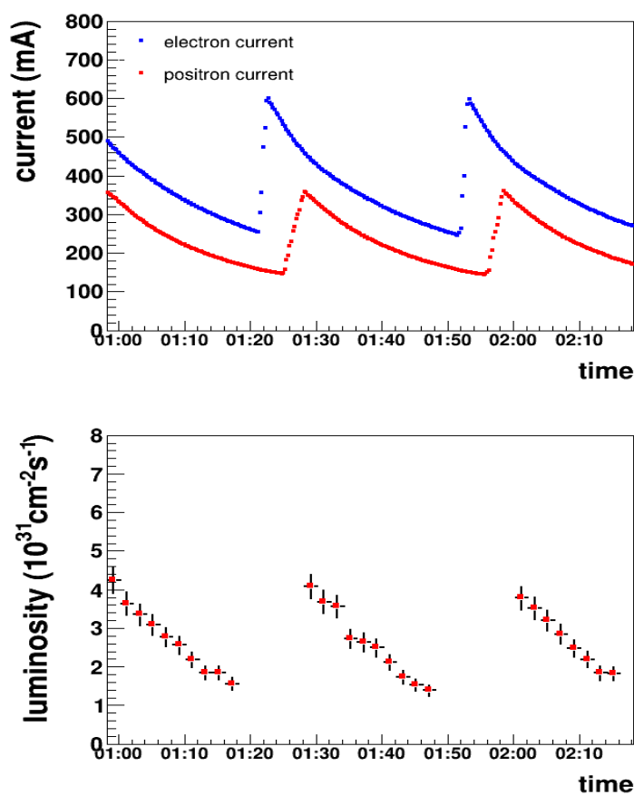
Figure 10. (upper) DAΦNE currents: electron (blue) and positron (red); (lower) measured luminosity — each point corresponds to 2 min of data taking.
