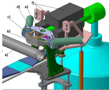
Fig. 1. The layout of the HPGe setup: a) beam pipe, b) luminometer, c) target, d) target holder, e) active part of the HPGe detector, f) lead shielding with the holder (figure done by C. Capoccia, LNF).
